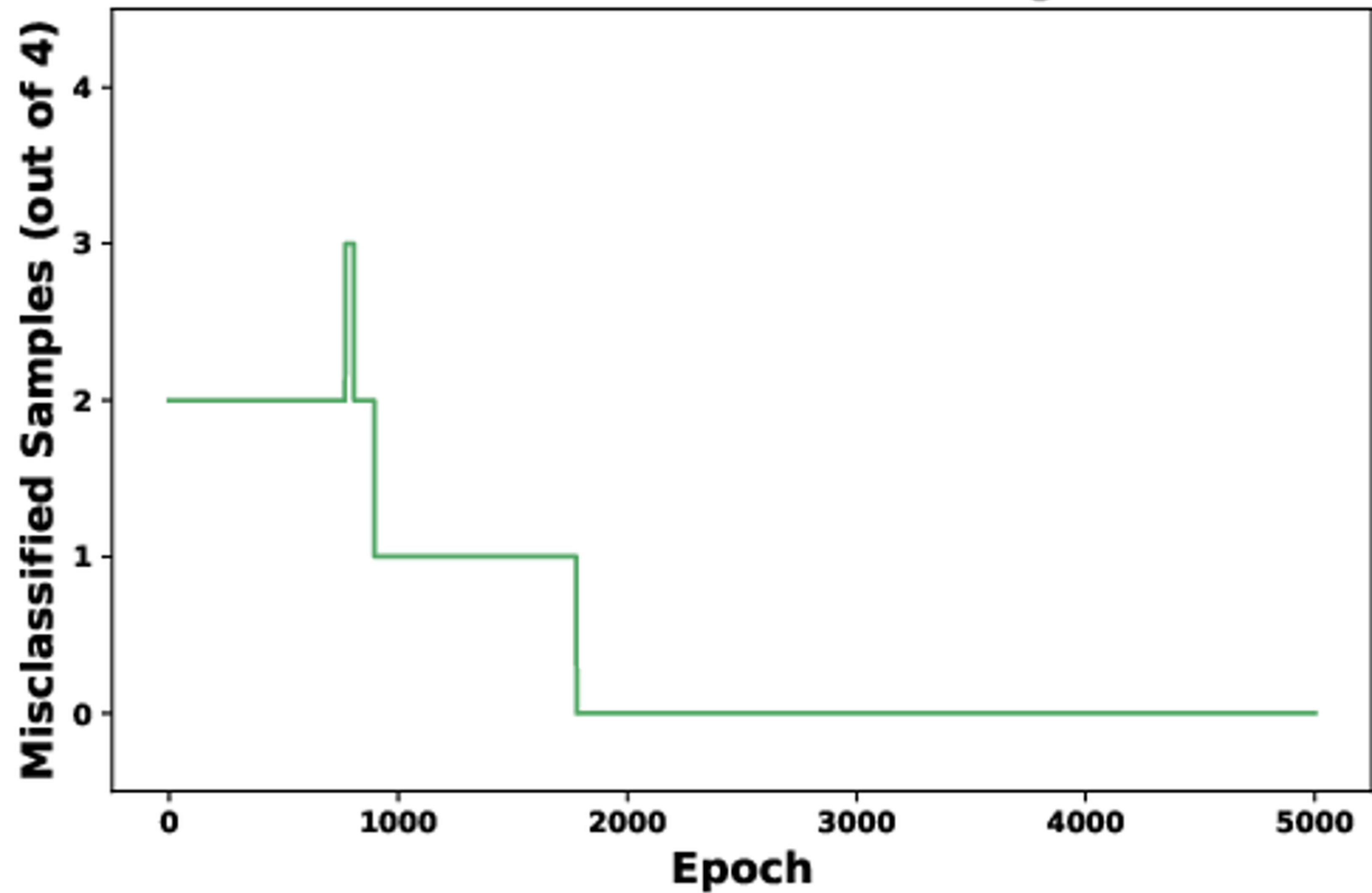
MLP Trained on XOR -- Convergence
